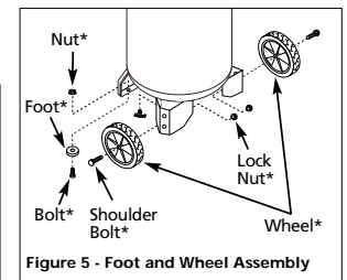
Figure 5 - Foot and Wheel Assembly
