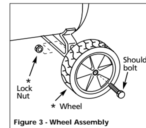
Figure 3 - Wheel Assembly
